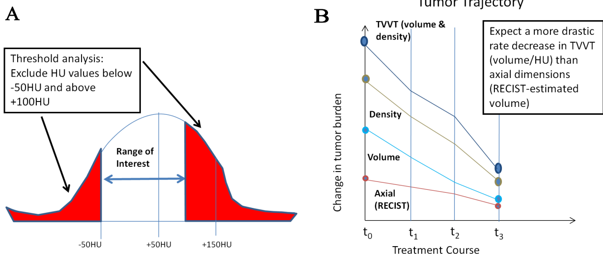
Figure 3A: Histograms can be used to calculate volumetric shifts in tumor composition and differentiate between necrotic and viable areas. Such use of thresholding can exclude areas not representative of tissues of interest (e.g., by excluding values over 100 Hounsfield units (HU) for calcifications and under -50HU for fat and artifact) giving a more comprehensive overall picture of tumor burden shift. B : Theoretical graphic representation of tumor trajectory over time in a
